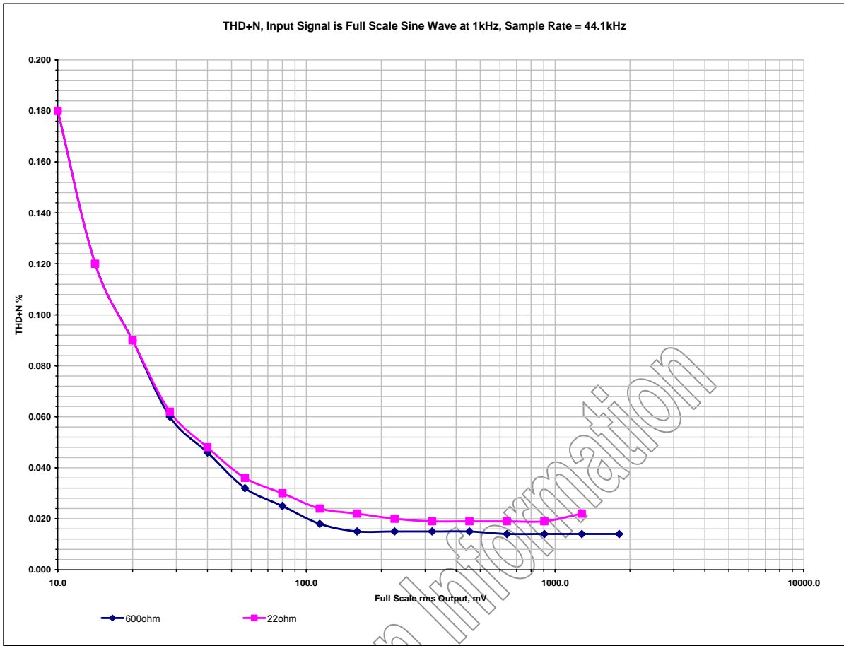
Figure 9.8: THD+N
