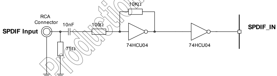
Figure 8.26: Example Circuit for SPDIF Interface with Coaxial Input
