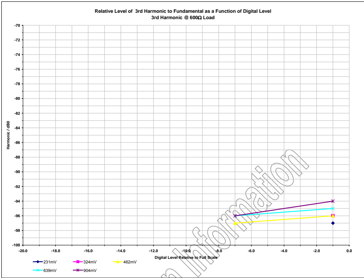
Figure 9.2: Relative Level of 3rd Harmonic to Fundamental, P L = 600Ω
