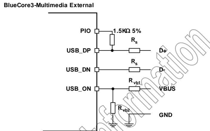
Figure 8.23: USB Connections for Self-Powered Mode
